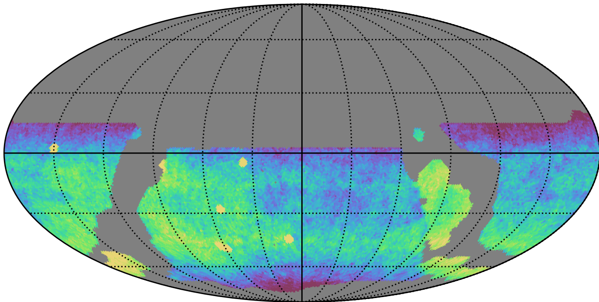
weather_cloudso12v3.4_10yrs WFD g band: CoaddM5
