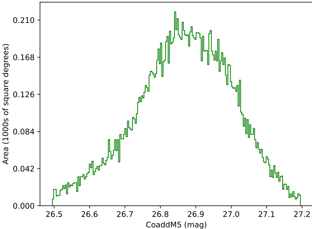
weather_cloudso12v3.4_10yrs WFD g band: CoaddM5
