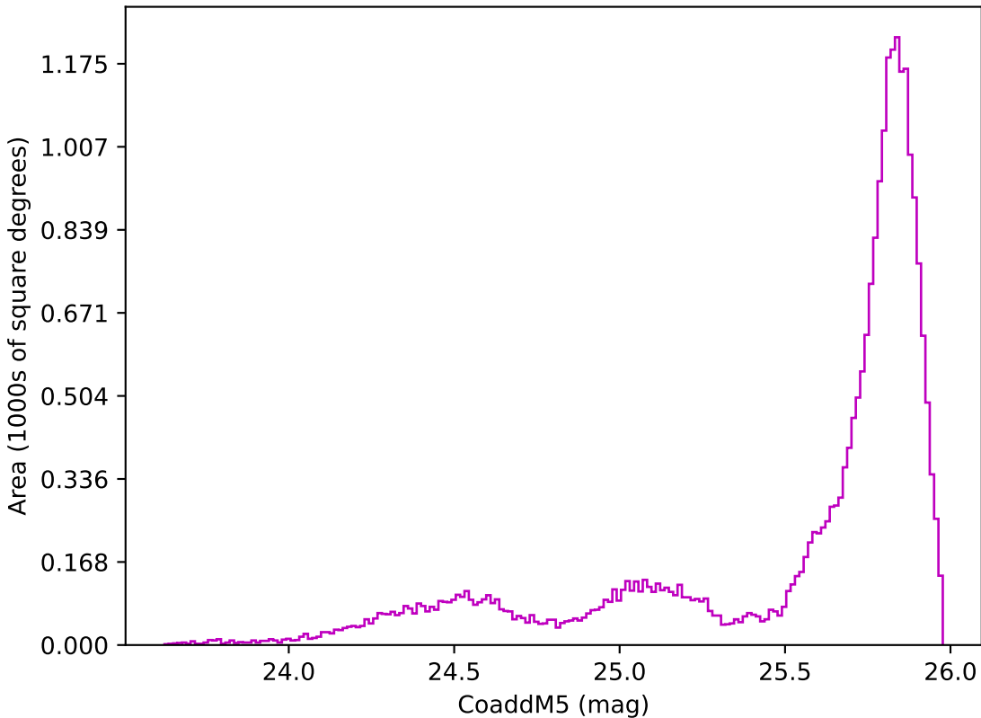
weather_cloudso12v3.4_10yrs All sky z band: CoaddM5
