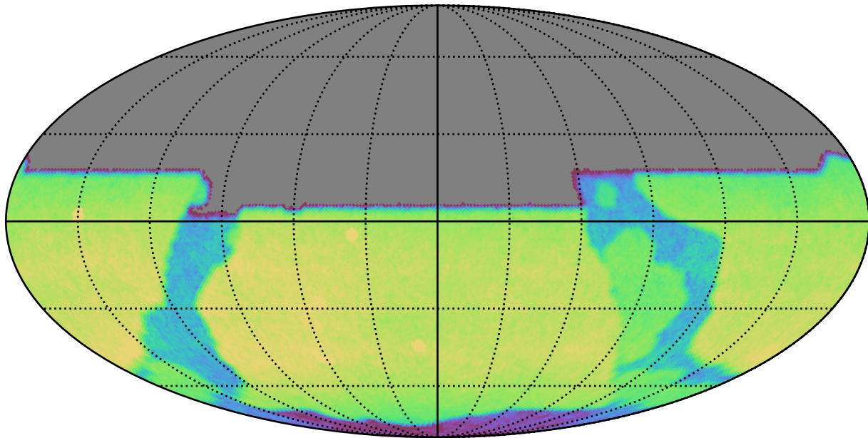
weather_cloudso12v3.4_10yrs All sky y band: CoaddM5
