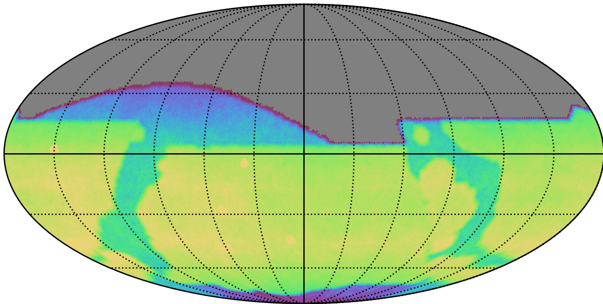
weather_cloudso12v3.4_10yrs All sky r band: CoaddM5
