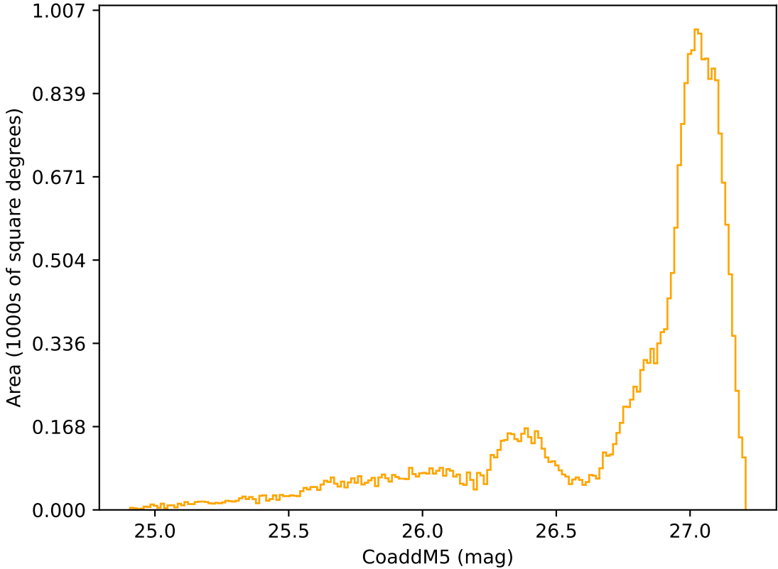
weather_cloudso12v3.4_10yrs All sky r band: CoaddM5
