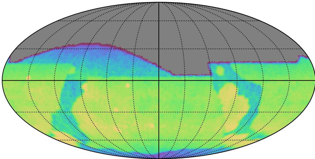
weather_cloudso12v3.4_10yrs All sky g band: CoaddM5
