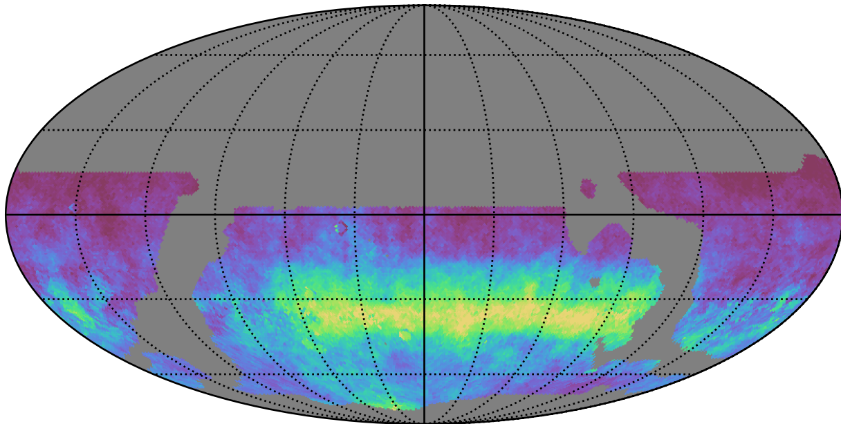
weather_cloudso12v3.4_10yrs WFD z band: AngleRms rotSkyPos
