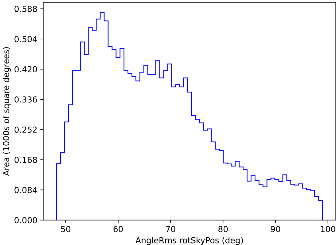
weather_cloudso12v3.4_10yrs WFD z band: AngleRms rotSkyPos
