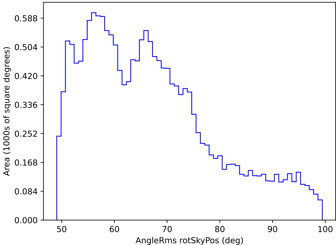
weather_cloudso12v3.4_10yrs WFD all bands: AngleRms rotSkyPos
