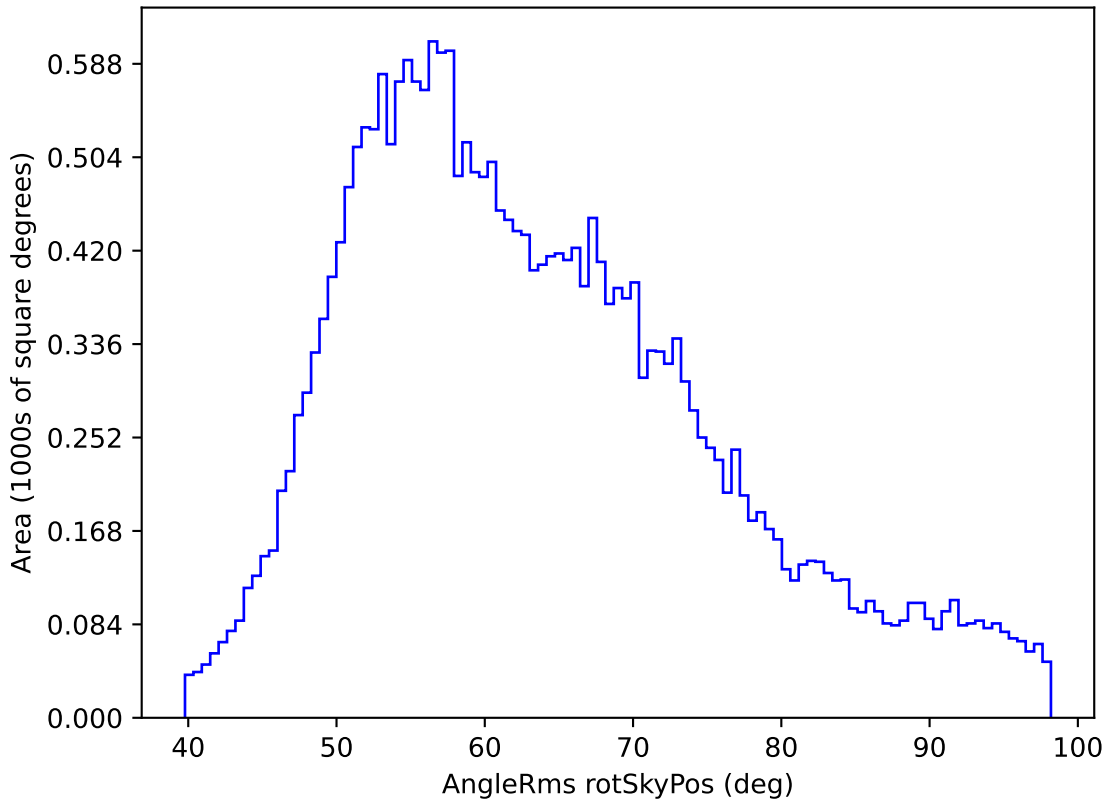
weather_cloudso12v3.4_10yrs All sky z band: AngleRms rotSkyPos
