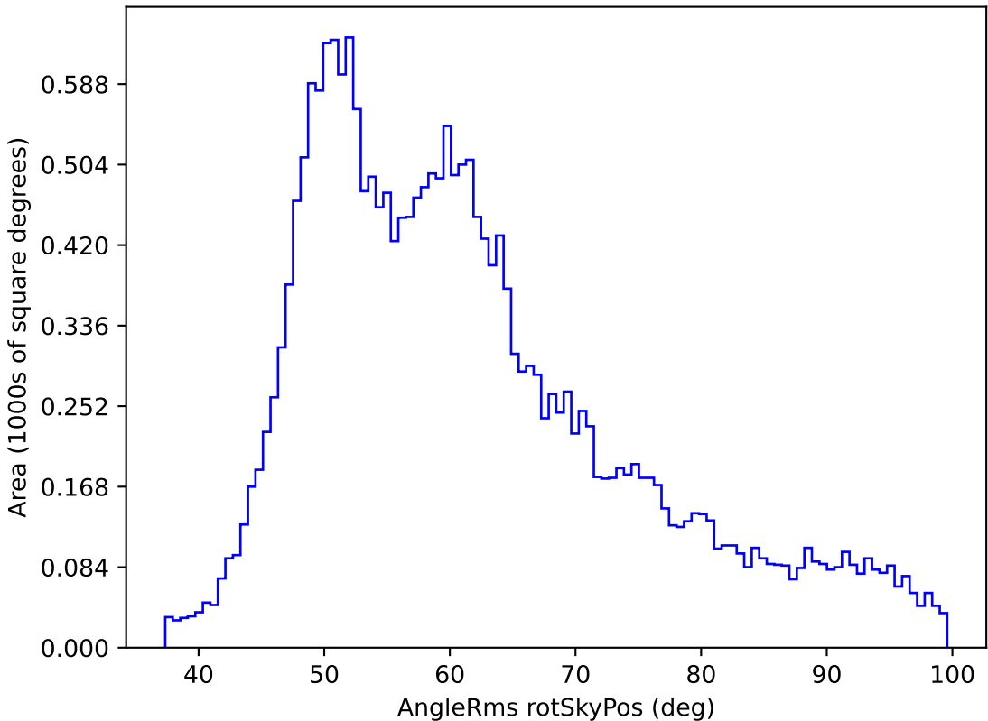
weather_cloudso12v3.4_10yrs All sky y band: AngleRms rotSkyPos
