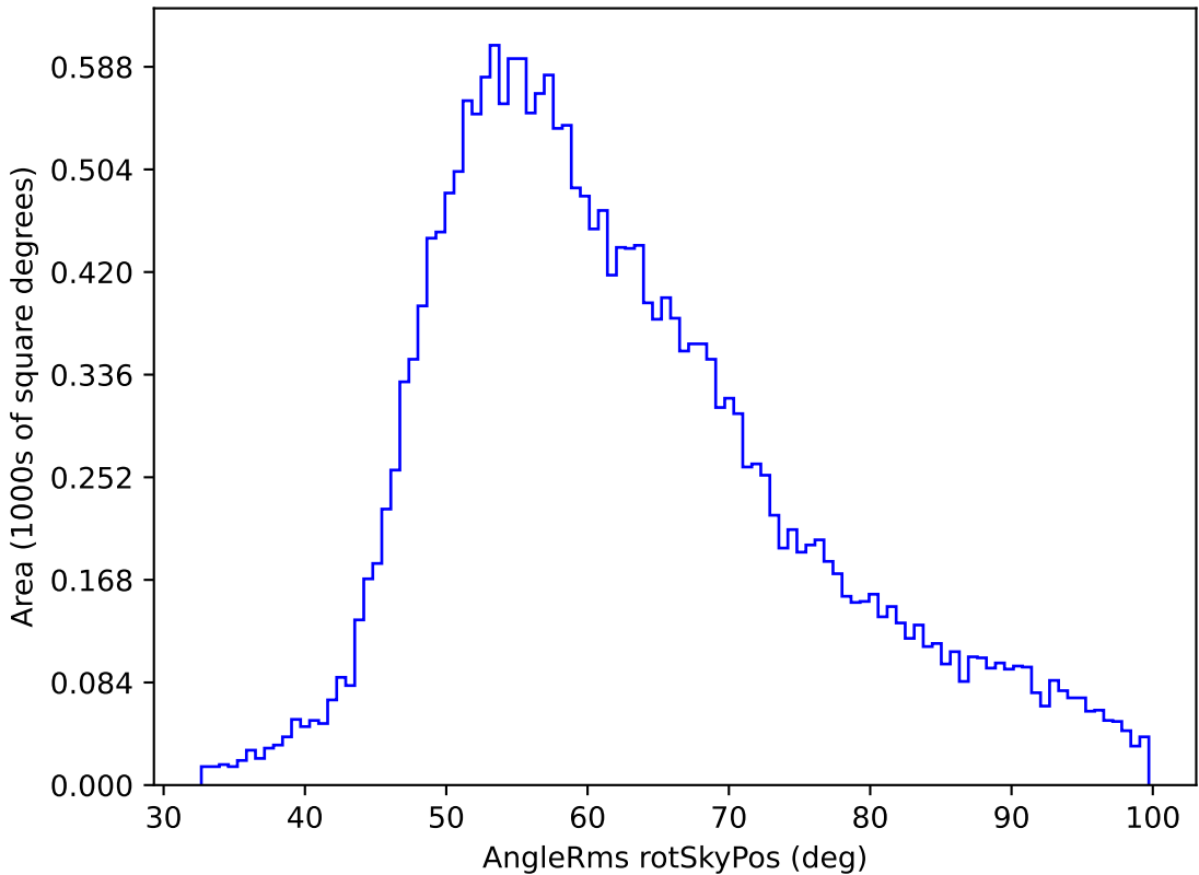
weather_cloudso12v3.4_10yrs All sky u band: AngleRms rotSkyPos
