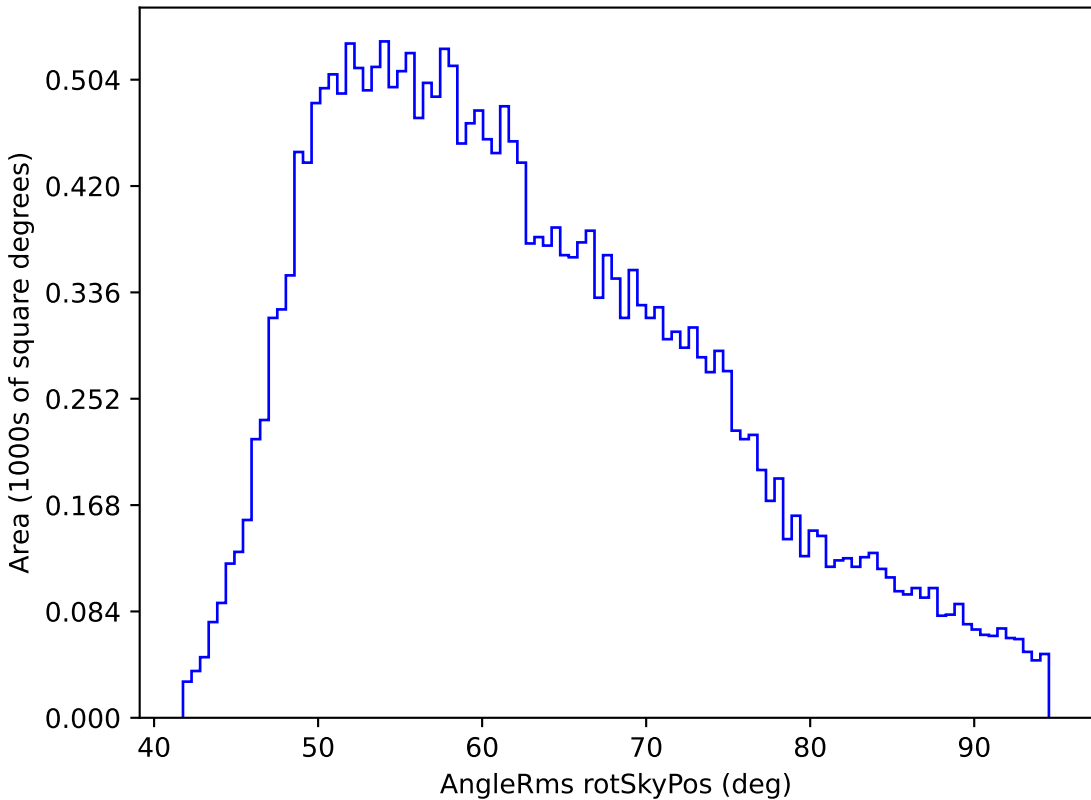
weather_cloudso12v3.4_10yrs All sky i band: AngleRms rotSkyPos
