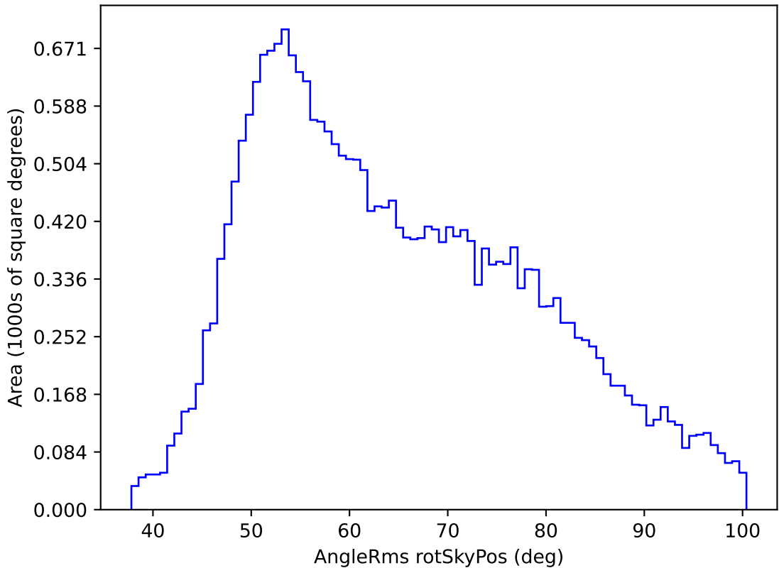
weather_cloudso12v3.4_10yrs All sky g band: AngleRms rotSkyPos
