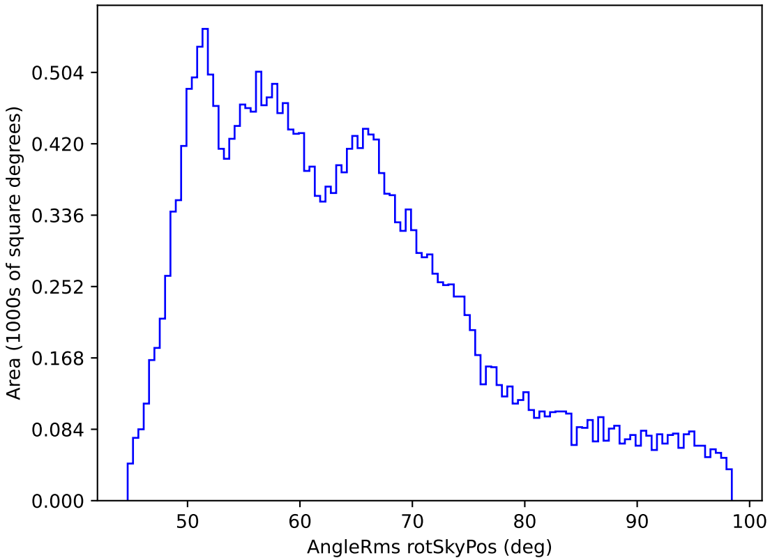
weather_cloudso12v3.4_10yrs All sky all bands: AngleRms rotSkyPos
