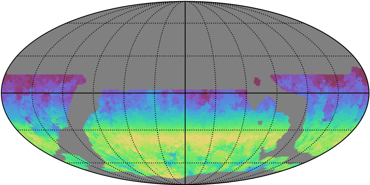
weather_cloudso12v3.4_10yrs WFD z band: AngleRange rotSkyPos
