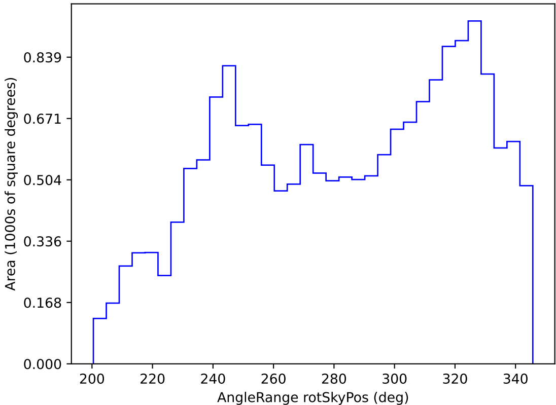
weather_cloudso12v3.4_10yrs WFD z band: AngleRange rotSkyPos
