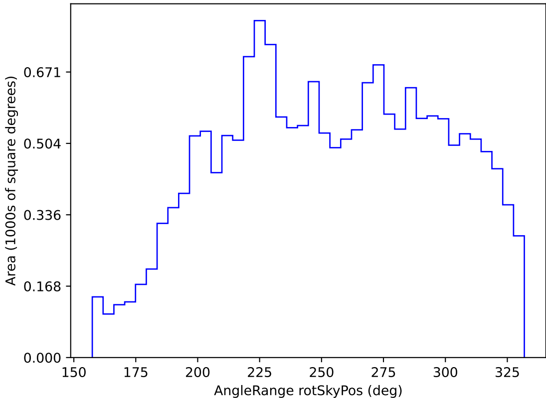
weather_cloudso12v3.4_10yrs WFD u band: AngleRange rotSkyPos
