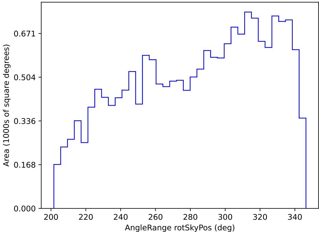
weather_cloudso12v3.4_10yrs WFD r band: AngleRange rotSkyPos
