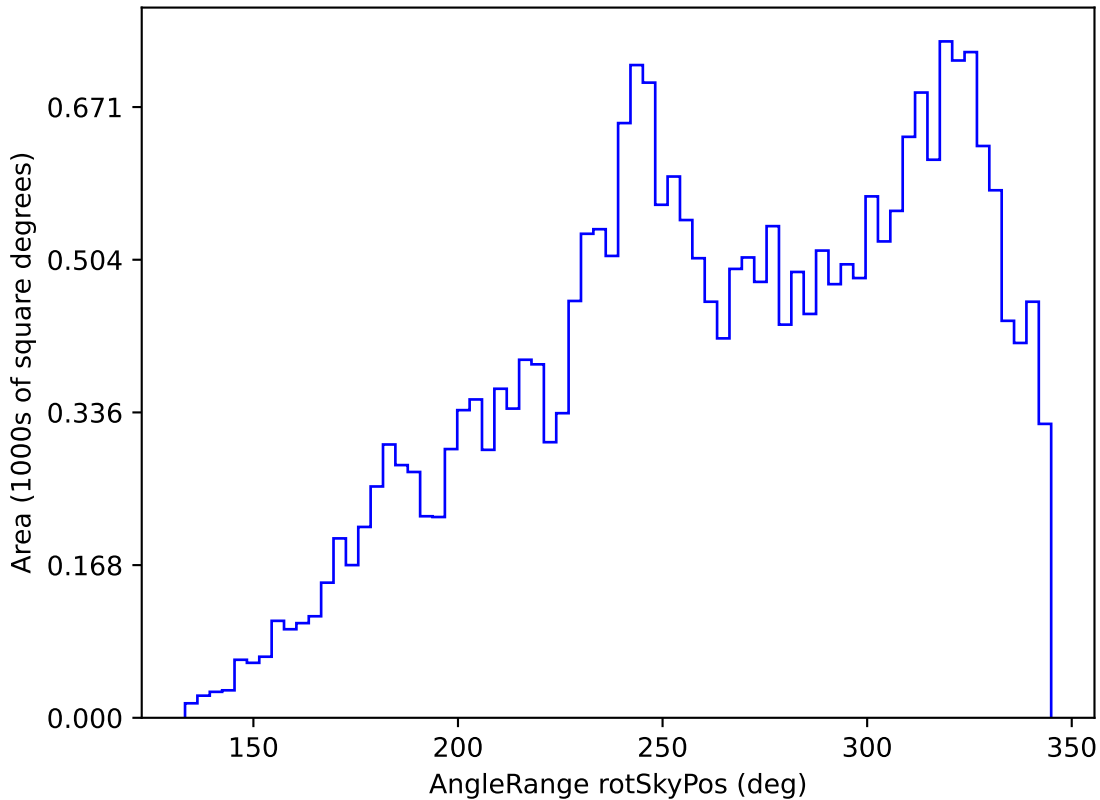
weather_cloudso12v3.4_10yrs All sky z band: AngleRange rotSkyPos
