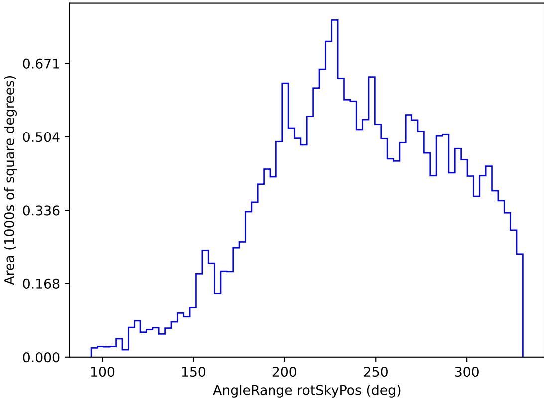
weather_cloudso12v3.4_10yrs All sky u band: AngleRange rotSkyPos
