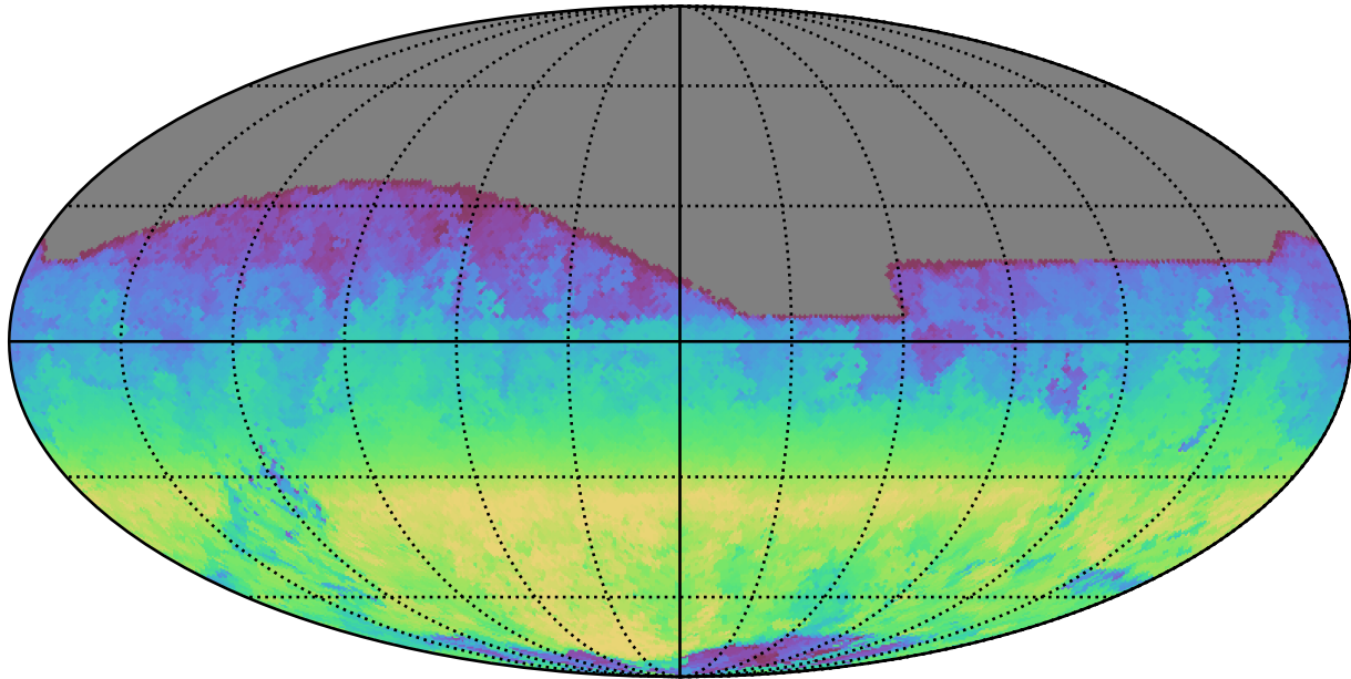
weather_cloudso12v3.4_10yrs All sky r band: AngleRange rotSkyPos
