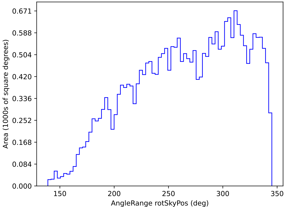
weather_cloudso12v3.4_10yrs All sky r band: AngleRange rotSkyPos
