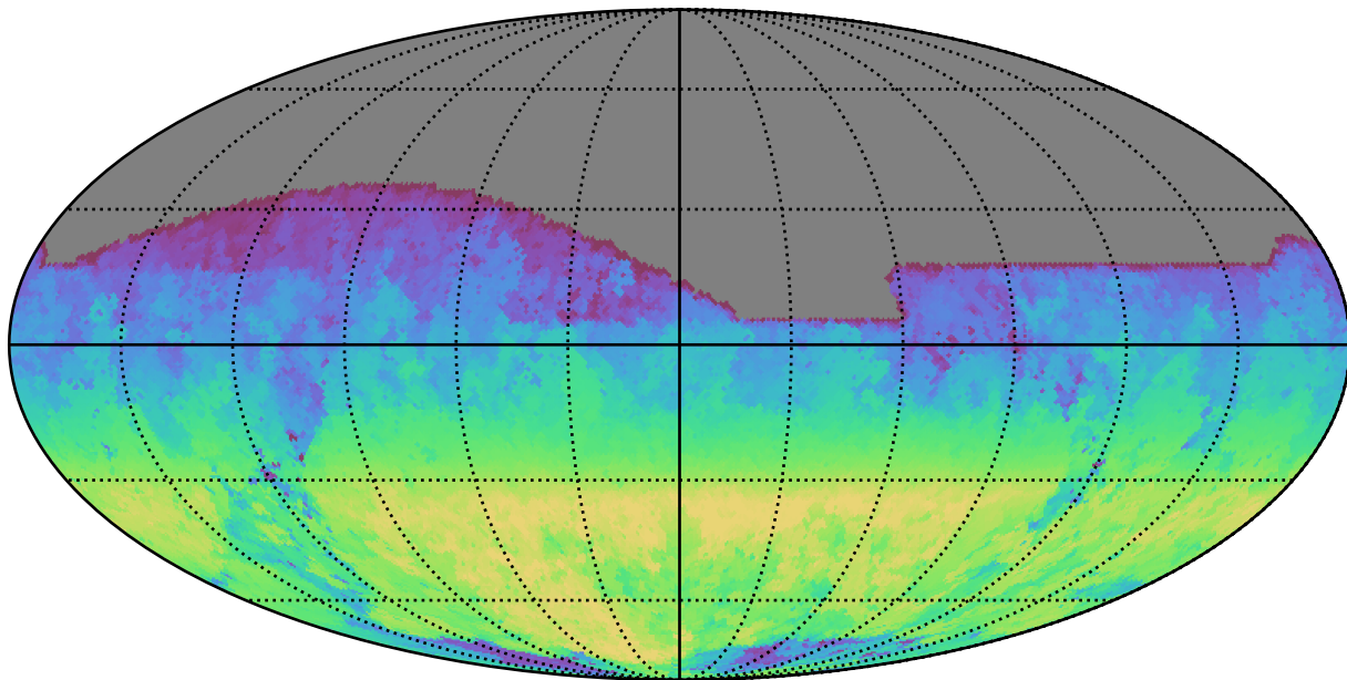
weather_cloudso12v3.4_10yrs All sky i band: AngleRange rotSkyPos
