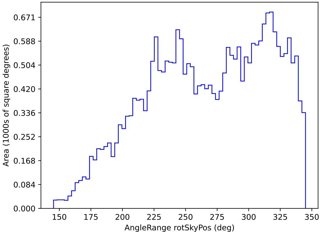
weather_cloudso12v3.4_10yrs All sky i band: AngleRange rotSkyPos
