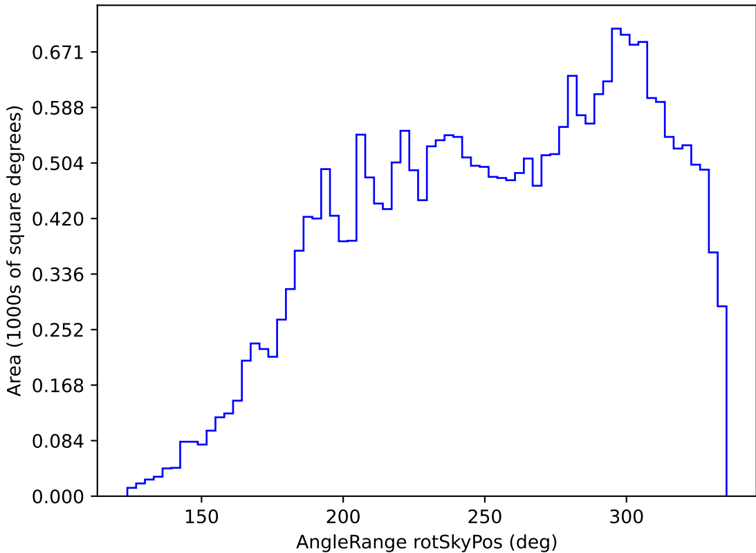
weather_cloudso12v3.4_10yrs All sky g band: AngleRange rotSkyPos
