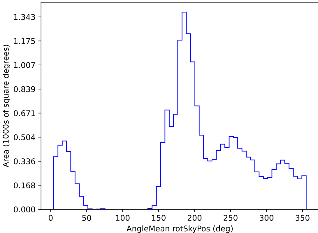
weather_cloudso12v3.4_10yrs WFD y band: AngleMean rotSkyPos
