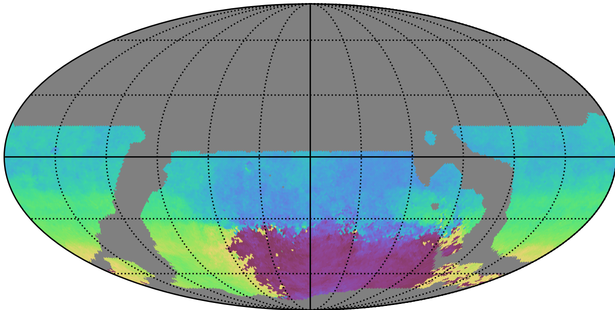
weather_cloudso12v3.4_10yrs WFD u band: AngleMean rotSkyPos
