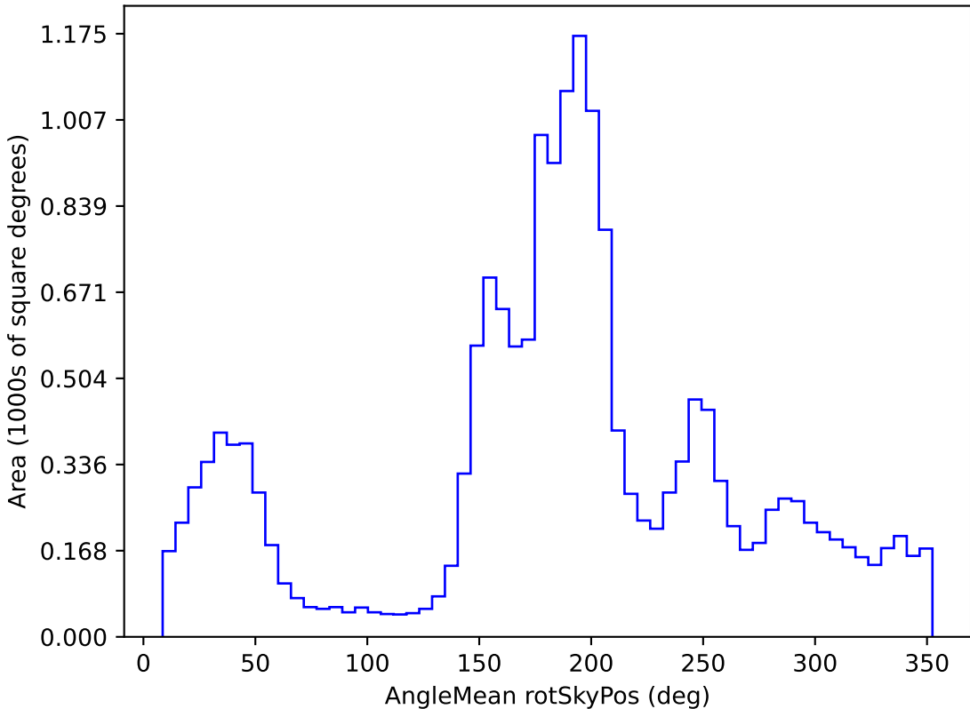
weather_cloudso12v3.4_10yrs WFD u band: AngleMean rotSkyPos
