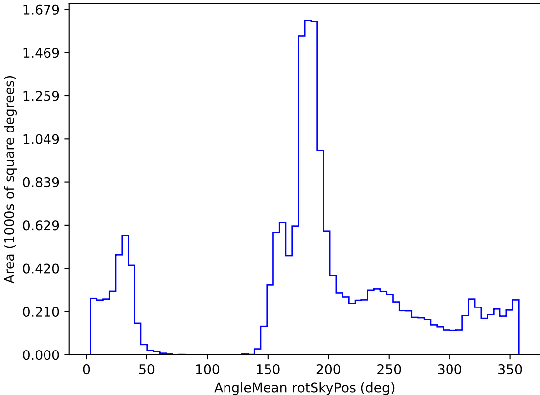
weather_cloudso12v3.4_10yrs WFD r band: AngleMean rotSkyPos
