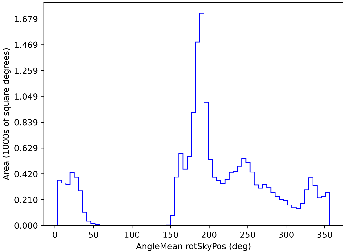
weather_cloudso12v3.4_10yrs WFD i band: AngleMean rotSkyPos
