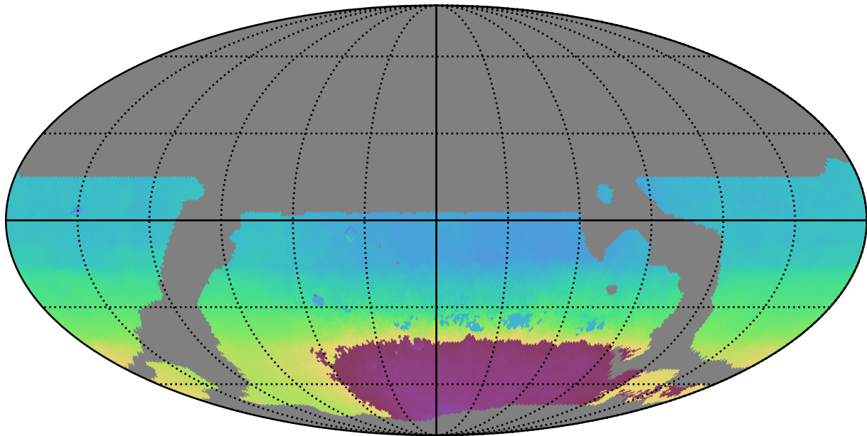
weather_cloudso12v3.4_10yrs WFD all bands: AngleMean rotSkyPos
