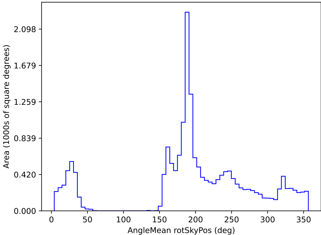
weather_cloudso12v3.4_10yrs WFD all bands: AngleMean rotSkyPos
