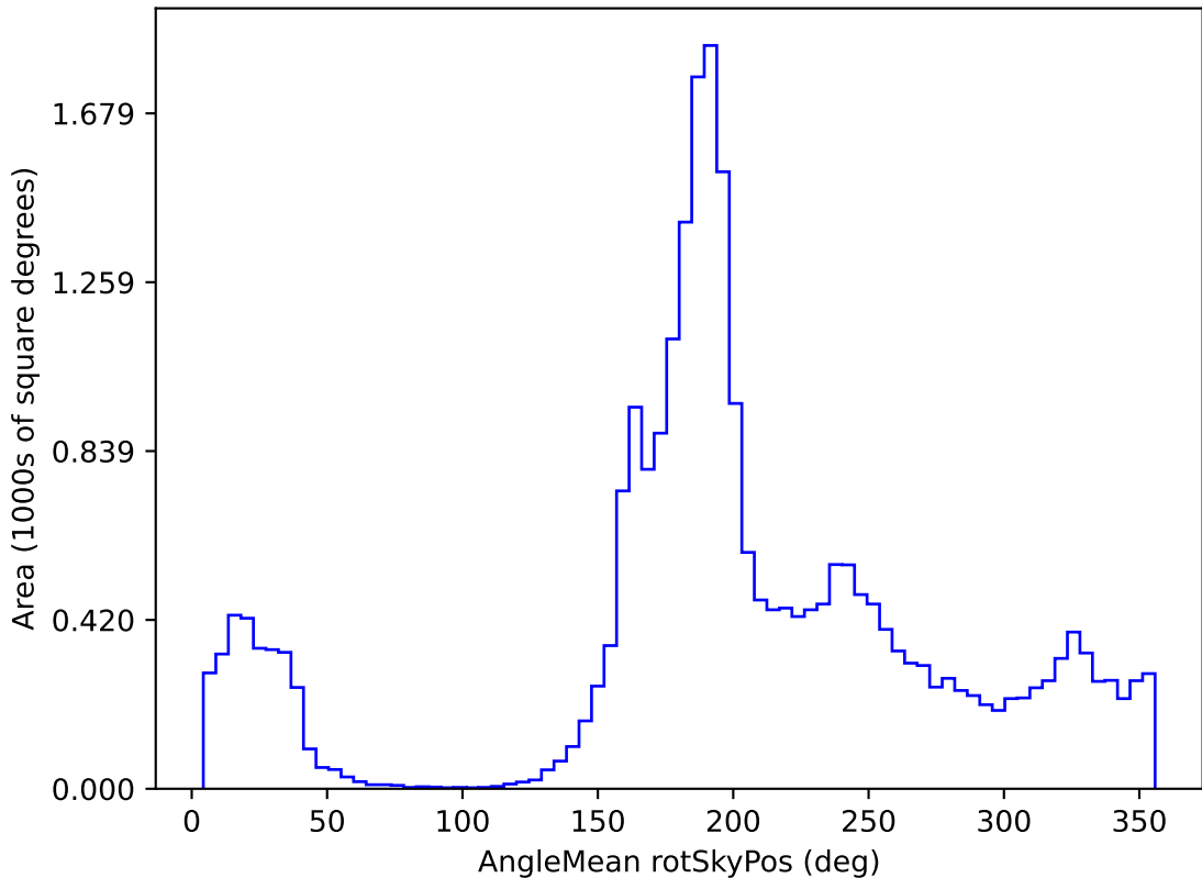
weather_cloudso12v3.4_10yrs All sky z band: AngleMean rotSkyPos
