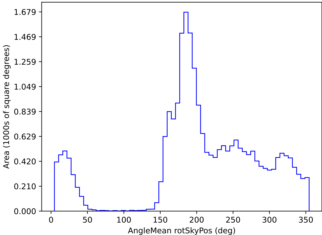
weather_cloudso12v3.4_10yrs All sky y band: AngleMean rotSkyPos
