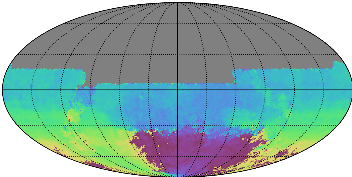
weather_cloudso12v3.4_10yrs All sky u band: AngleMean rotSkyPos
