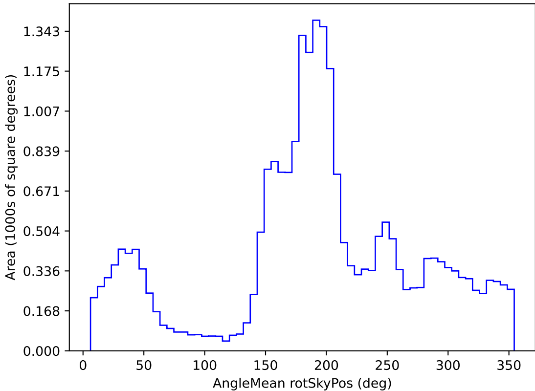
weather_cloudso12v3.4_10yrs All sky u band: AngleMean rotSkyPos
