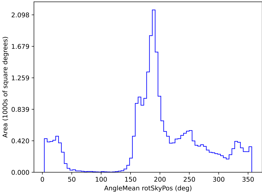
weather_cloudso12v3.4_10yrs All sky i band: AngleMean rotSkyPos
