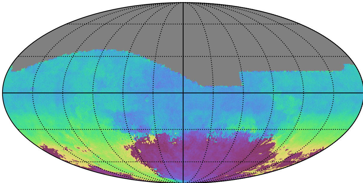
weather_cloudso12v3.4_10yrs All sky g band: AngleMean rotSkyPos
