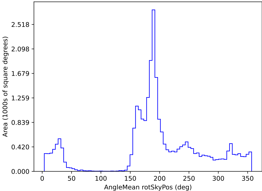
weather_cloudso12v3.4_10yrs All sky all bands: AngleMean rotSkyPos
