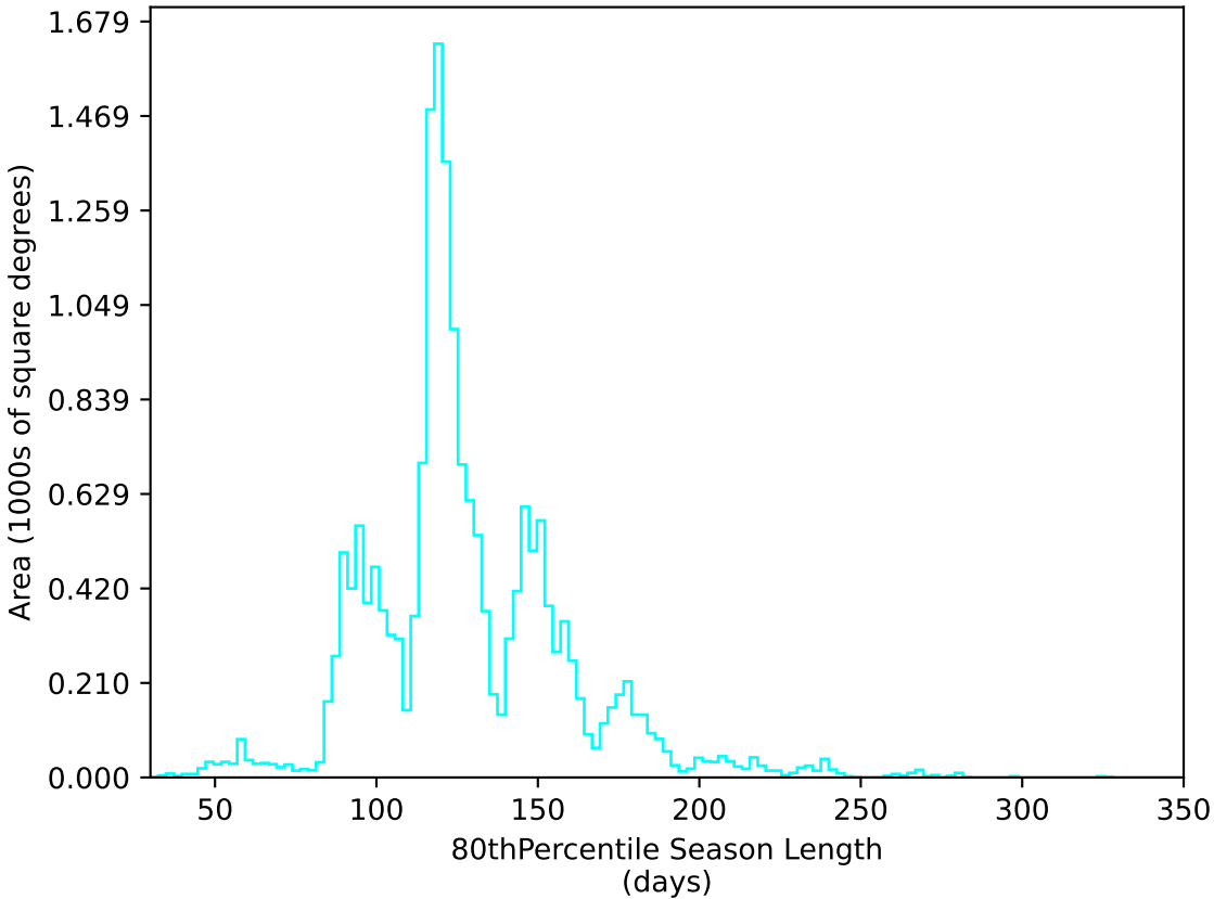
weather_cloudso12v3.4_10yrs WFD u band: 80thPercentile Season Length
