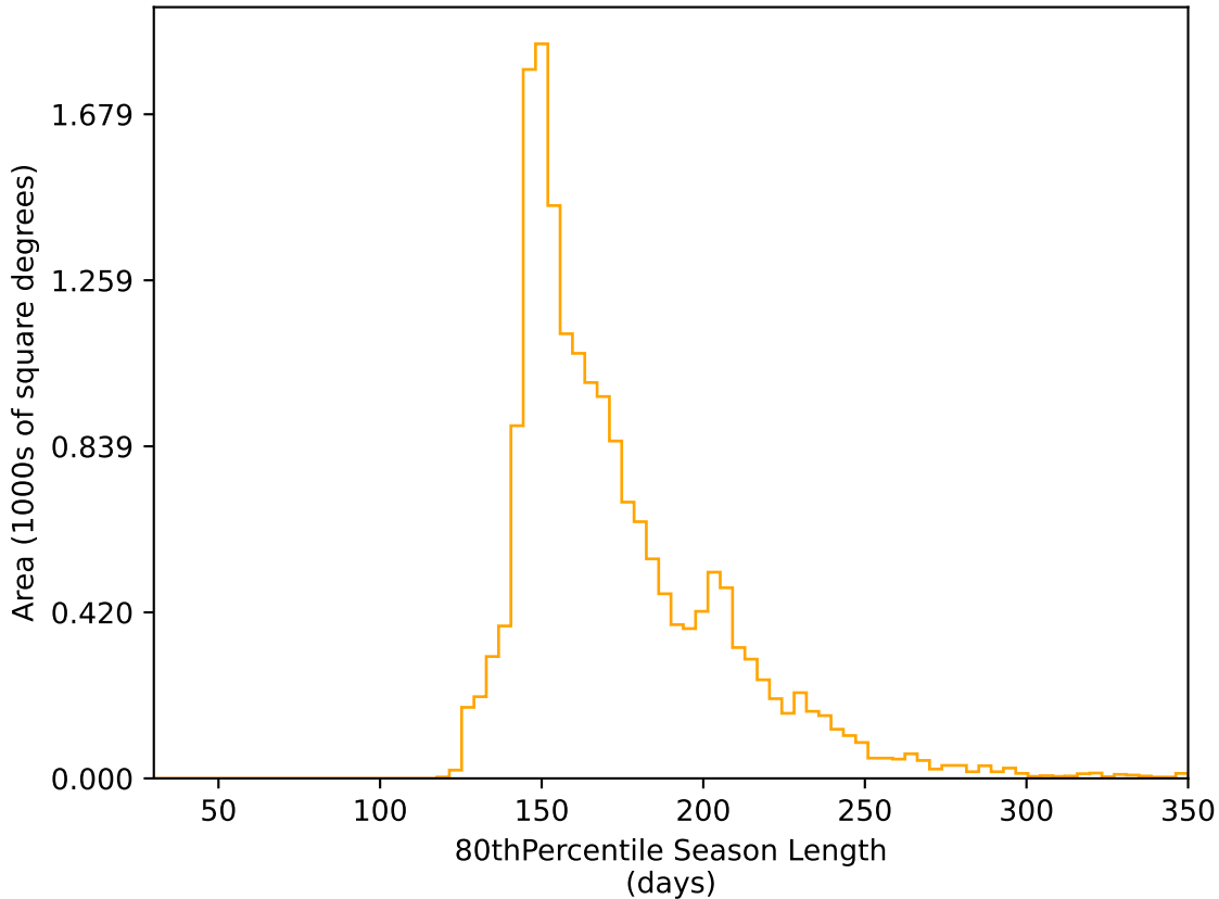
weather_cloudso12v3.4_10yrs WFD r band: 80thPercentile Season Length
