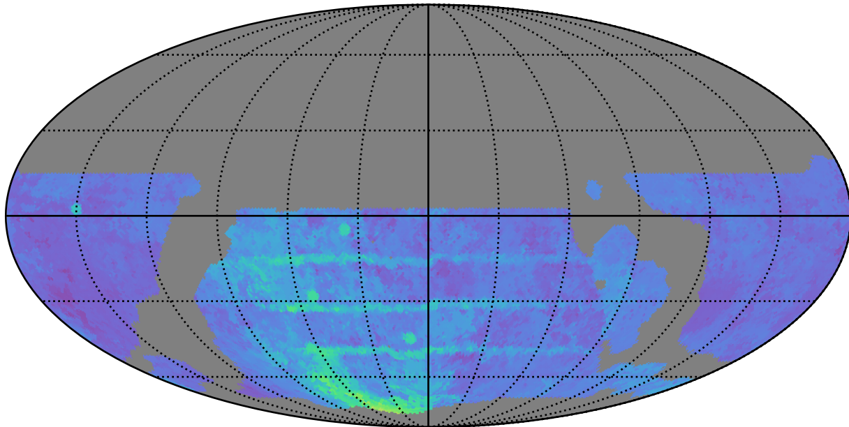
weather_cloudso12v3.4_10yrs WFD g band: 80thPercentile Season Length
