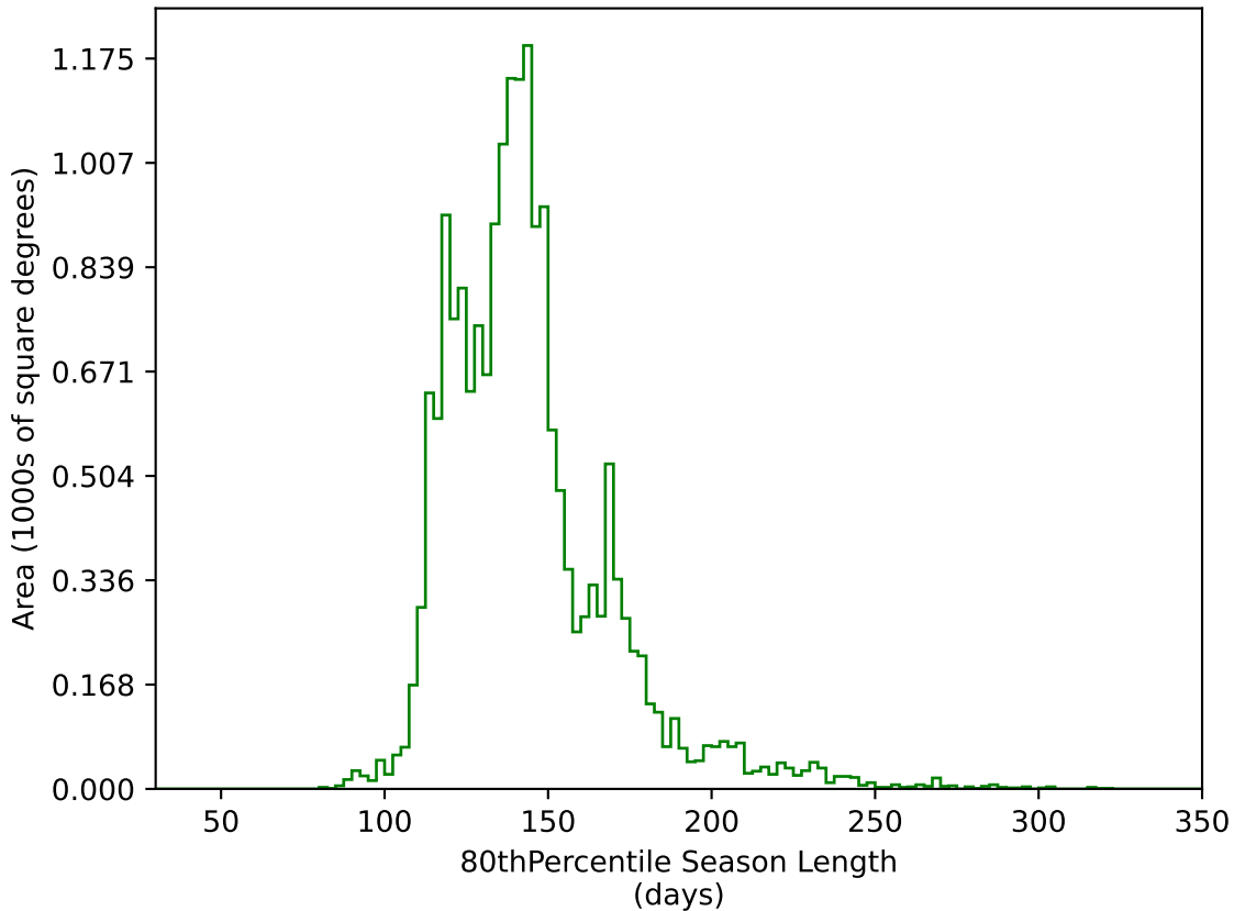
weather_cloudso12v3.4_10yrs WFD g band: 80thPercentile Season Length
