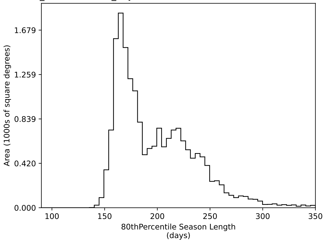
weather_cloudso12v3.4_10yrs WFD all bands: 80thPercentile Season Length
