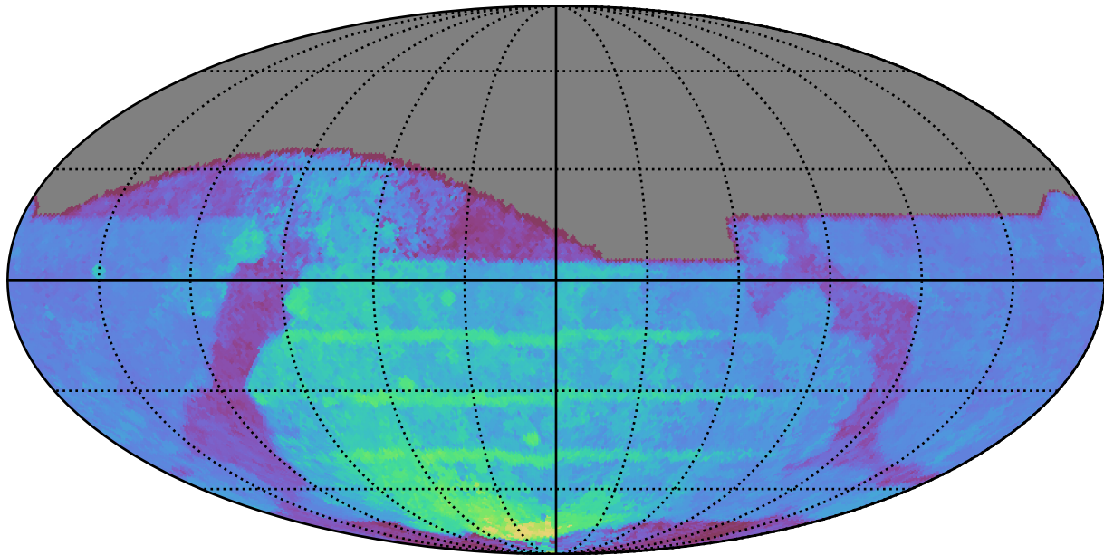
weather_cloudso12v3.4_10yrs All sky z band: 80thPercentile Season Length
