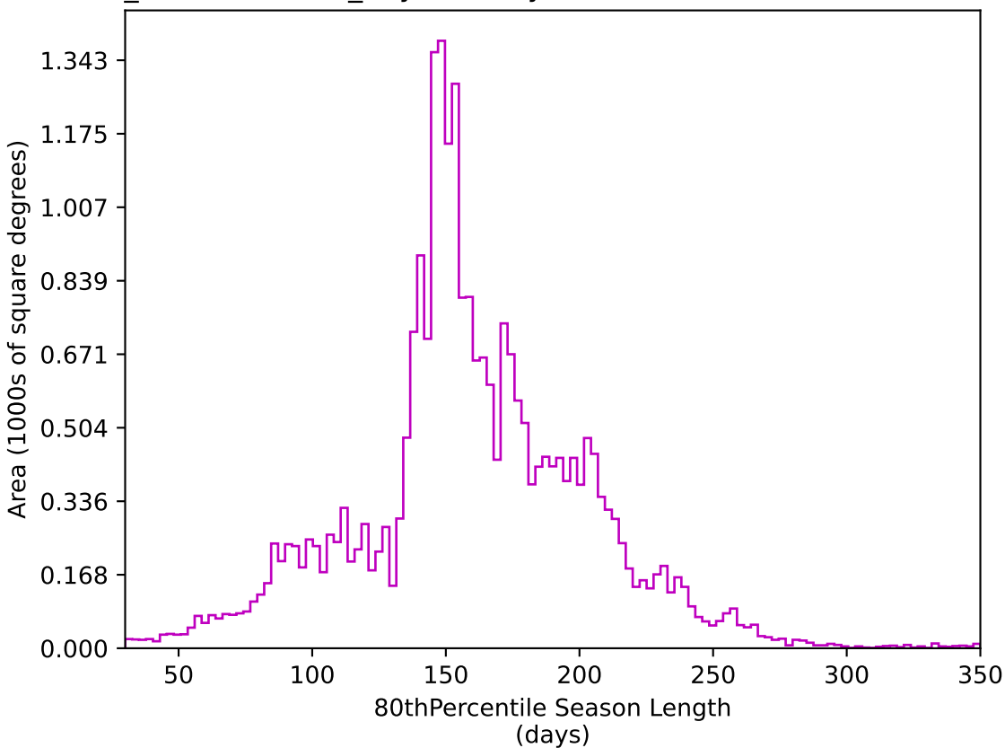
weather_cloudso12v3.4_10yrs All sky z band: 80thPercentile Season Length
