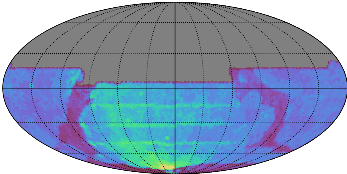
weather_cloudso12v3.4_10yrs All sky y band: 80thPercentile Season Length
