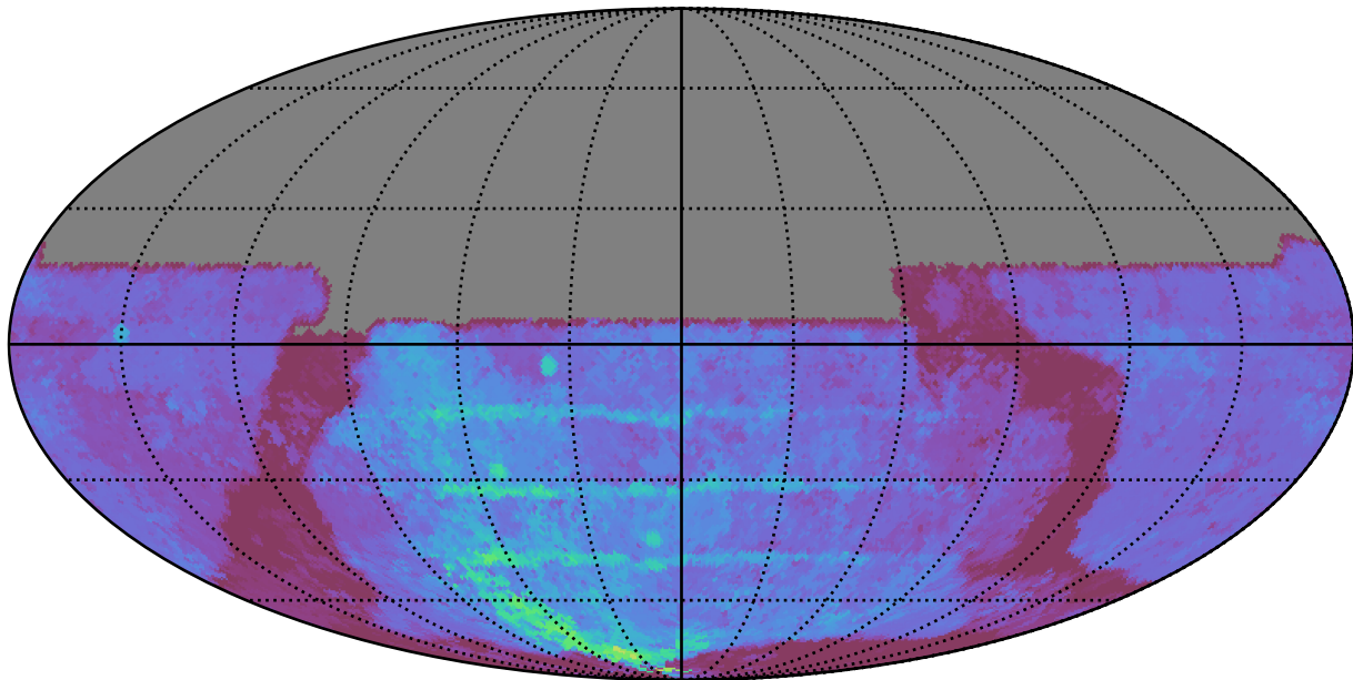
weather_cloudso12v3.4_10yrs All sky u band: 80thPercentile Season Length
